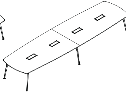
ELİPS TOPLANTI MASASI ELLIPTICAL MEETING TABLE L 480 W 130 H 75
