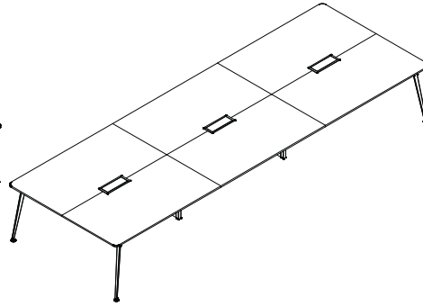
TOPLANTI MASASI MEETING TABLE L 480 / 540 / 600 W 165 H 75
