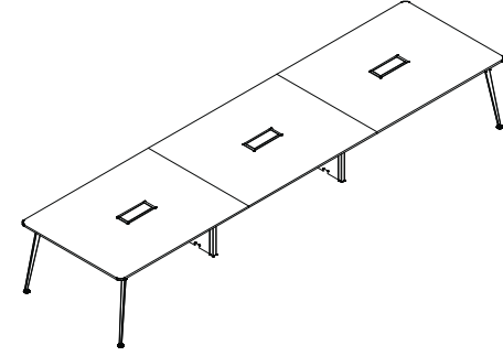
TOPLANTI MASASI MEETING TABLE L 320 / 360 / 400 W 125 H 75
