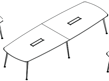
ELİPS TOPLANTI MASASI ELLIPTICAL MEETING TABLE L 400 W 130 H 75
